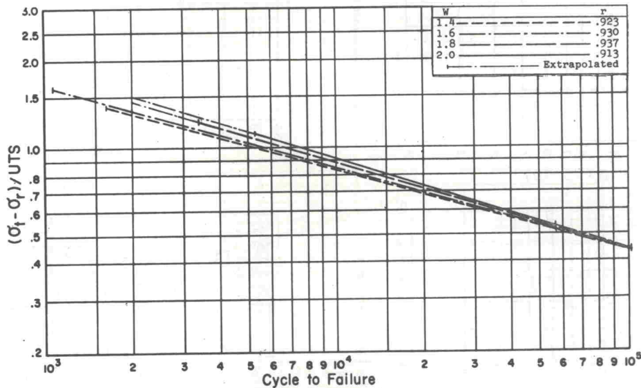
Fig. 7 Octahedral stress parameter versus cycles to failure
